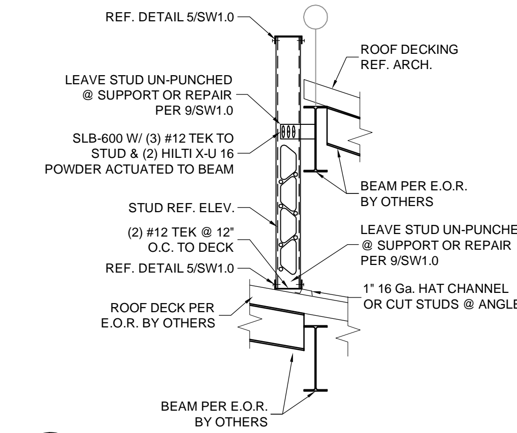
14 WALL @ SAW TOOTH N.T.S. 13/S-405
