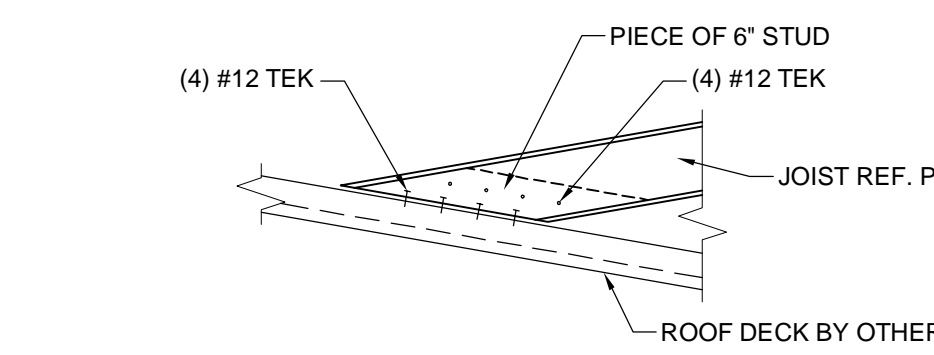
12 JOIST AT VALLEY N.T.S.
